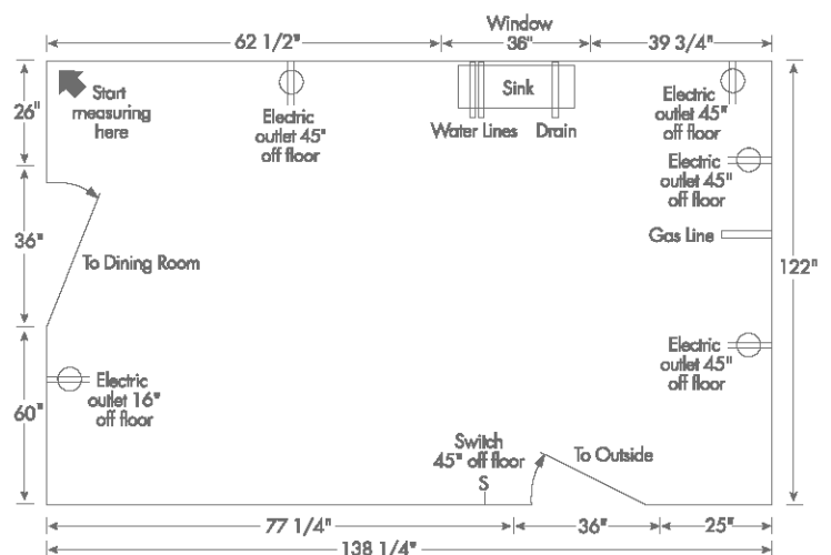
SAMPLE FLOOR PLAN HERE:
